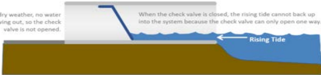
Figure 59: Graphic depiction of backflow preventer technology at stormwater outfall site (Image Source: City of Charelston, SC)
